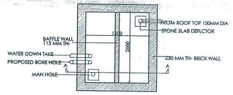
SECTION PLAN OF LINDE GROUND WATER TANK (2000X1800)
