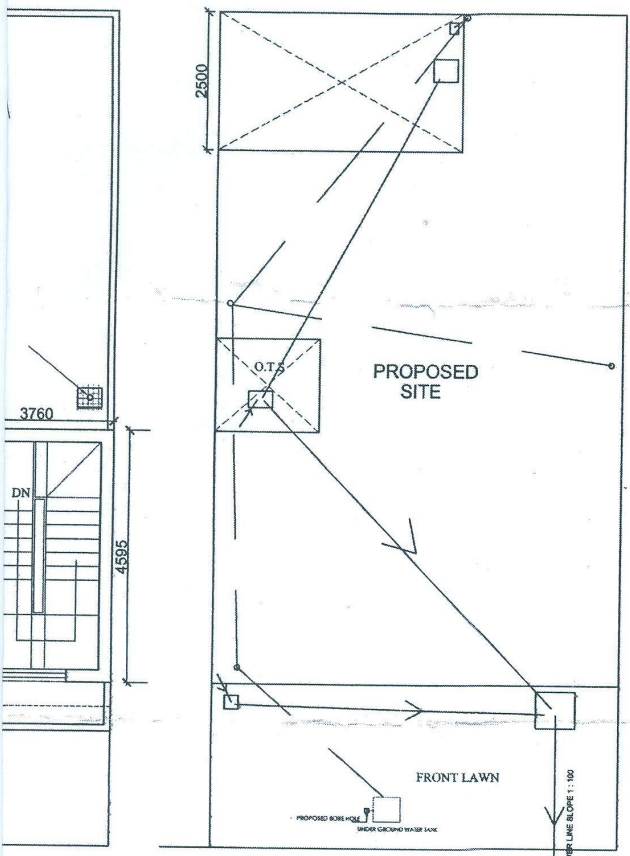
6.0 MT WIDE ROAD SITE PLAN AND RAIN WATER HARVESTING SCALE -1:100
