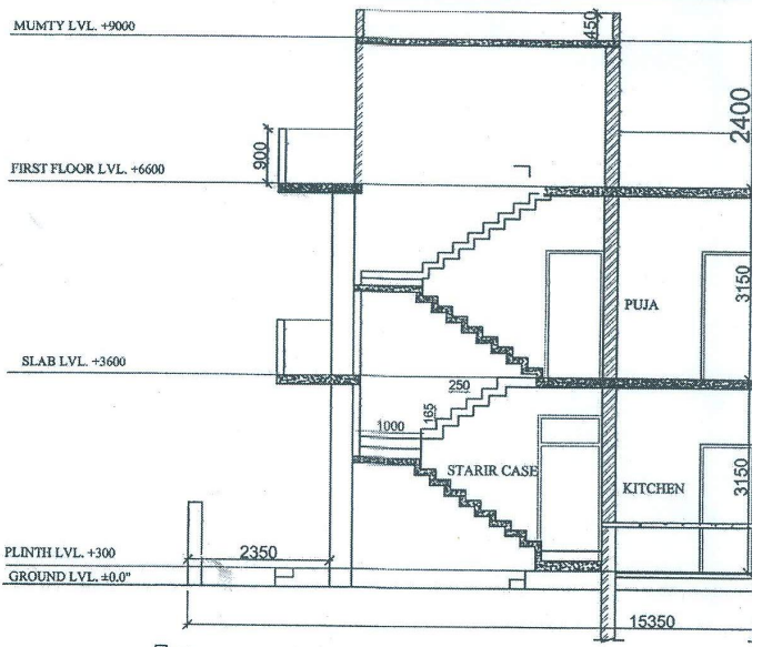
SECTION A SCALE
