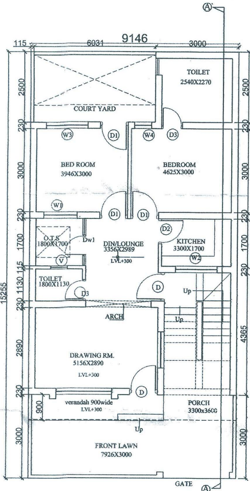
6.0 MT WIDE ROAD GROUND FLOOR PLAN SCALE=1:100
